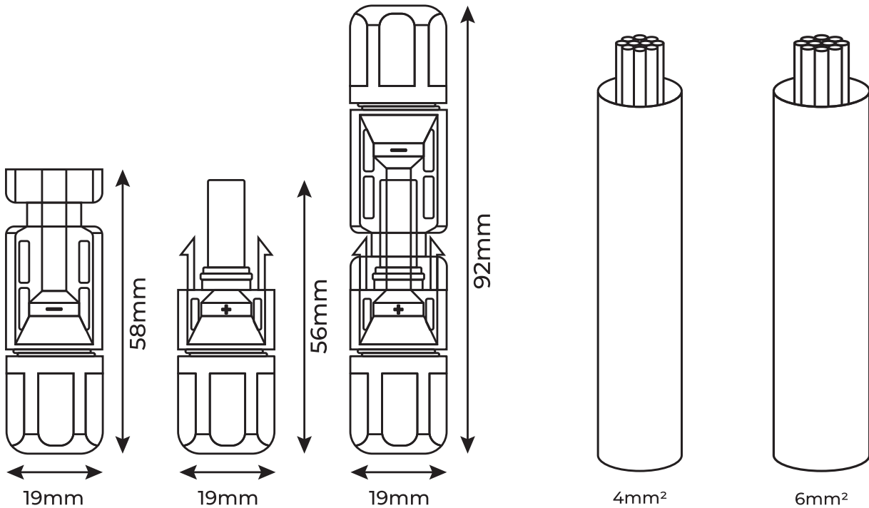
Solar Connectors
