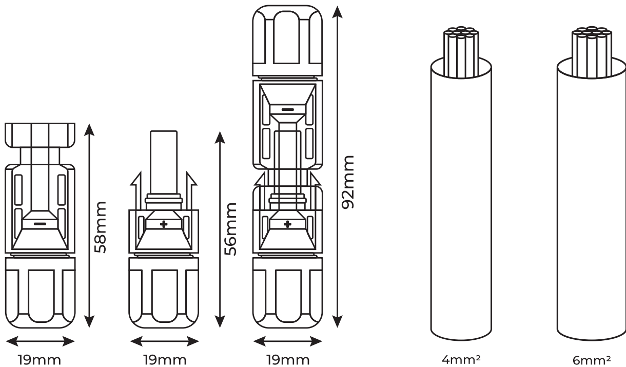
Solar Connectors
